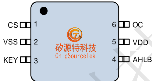
RM1281AST6A (SOT23-6)
