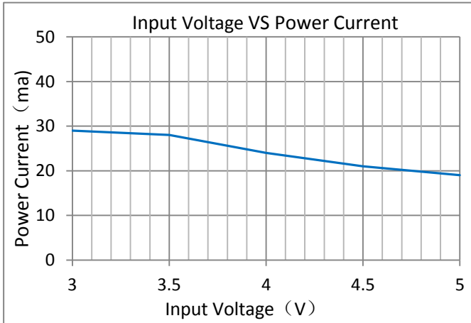
图5: Power Crrnt VS. Suppy Voltage
